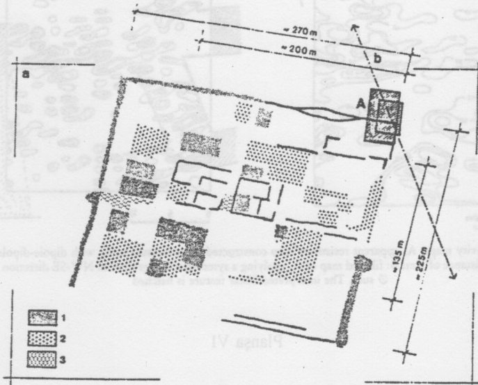
Fig. 3. Archaeological interpretation of Fig. 2. A: the geophysical test site; a: boundary of the polaroid picture; b: one time road which can be seen on the photo; 1: calcareous stains appearing sharply, presumably houses and fortress walls; 2: more dimly visible stains suggesting the presence of a building; 3: possible traces of roads of the camp
